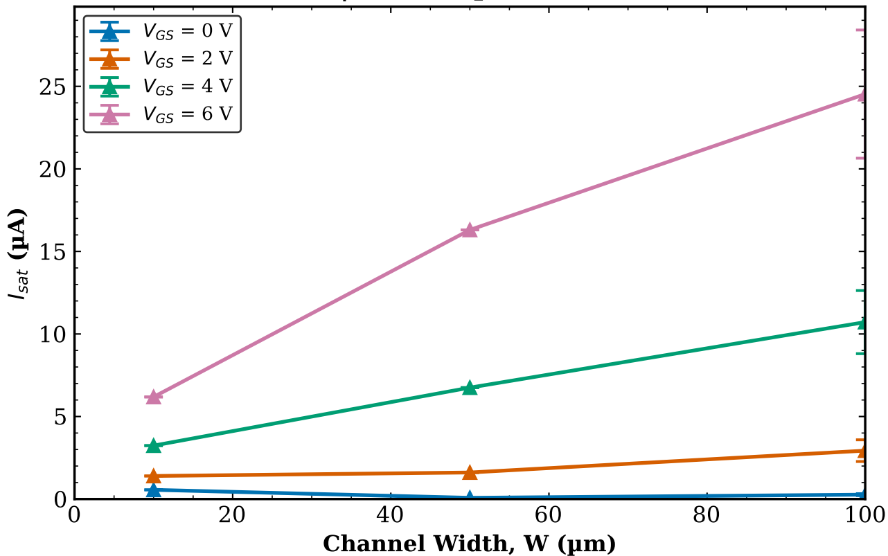
TFT3 Combined (Tr. 1 & 2) I_{sat} vs W | L = 40\text{ }\mu\text{m} (mean \pm std)
